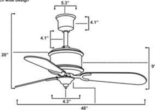
Size Chart Monarch wide Design
