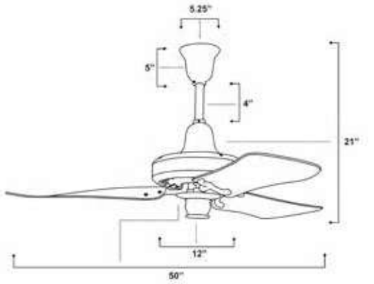
Size Chart Diva Heritage Wide Design
