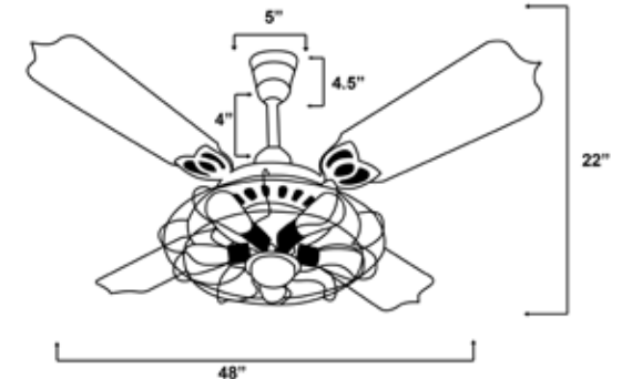
Size Chart Legend with light fan
