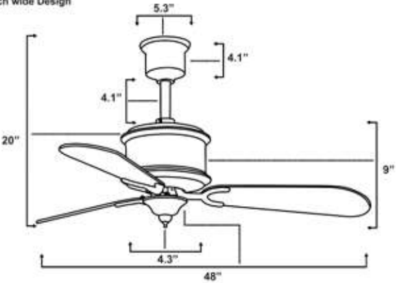
Size Chart Monarch wide Design
