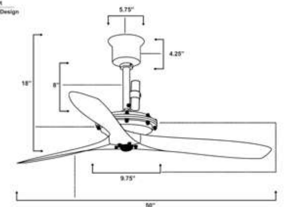
Size Chart Aviator 3 Design
